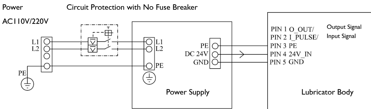
Power System Wiring diagram
